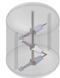
CFI Counter flow impeller
